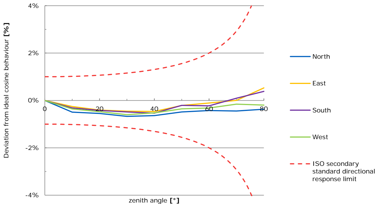
Figure 3 Directional response of a SR20 pyranometer of 4 azimuth angles, compared to secondary standard limits
