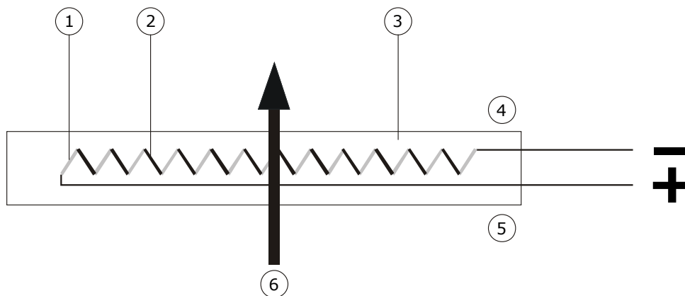
Figure 2.1 The general working principle of a heat flux sensor. The sensor inside FHF01 is a thermopile. A thermopile consists of a number of thermocouples, each consisting of two metal alloys marked 1 and 2, electrically connected in series. A single thermocouple generates an output voltage that is proportional to the temperature difference between its hot- and cold joints. Putting thermocouples in series amplifies the signal. In a heat flux sensor, the hot- and cold joints are located at the opposite sensor surfaces 4 and 5. In steady state, the heat flux 6 is a linear function of the temperature difference across the sensor and the average thermal conductivity of the sensor body, 3. The thermopile generates a voltage output proportional to the heat flux through the sensor. The exact sensitivity of the sensor is determined at the manufacturer by calibration, and can be found on the product certificate that is supplied with each sensor.
