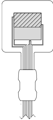
Figure 5.3.3.1 Picture of FHF01 with top 50 % highlighted (total sensing area is shaded grey; top 50 % is accentuated by diagonal lines in this image)
