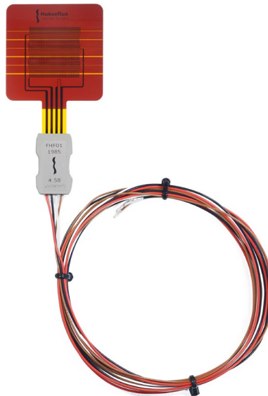
Figure 1.2.1 FHF01 with bundled wiring; FHF01's serial number and sensitivity are visible on the strain relief block
