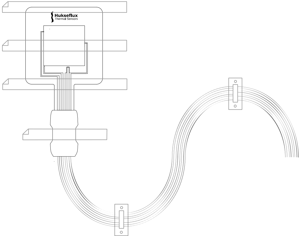
Figure 5.1.1 Installation of FHF01 using tape to fixate the sensor and the strain relief block. Extra strain relief of the wire is provided using cable tie mounts equipped with double sided tape as adhesive. As indicated in Table 5.1.1, tapes fixating the sensor are preferably taped over the passive guard area. In this case a third tape (in the middle) is added for extra support. Please note the Hukseflux logo is readable in this image; this indicates that we are viewing the front side and that the other side, the back side, is attached on the object on which the sensor is mounted, as explained in Chapter 2.
