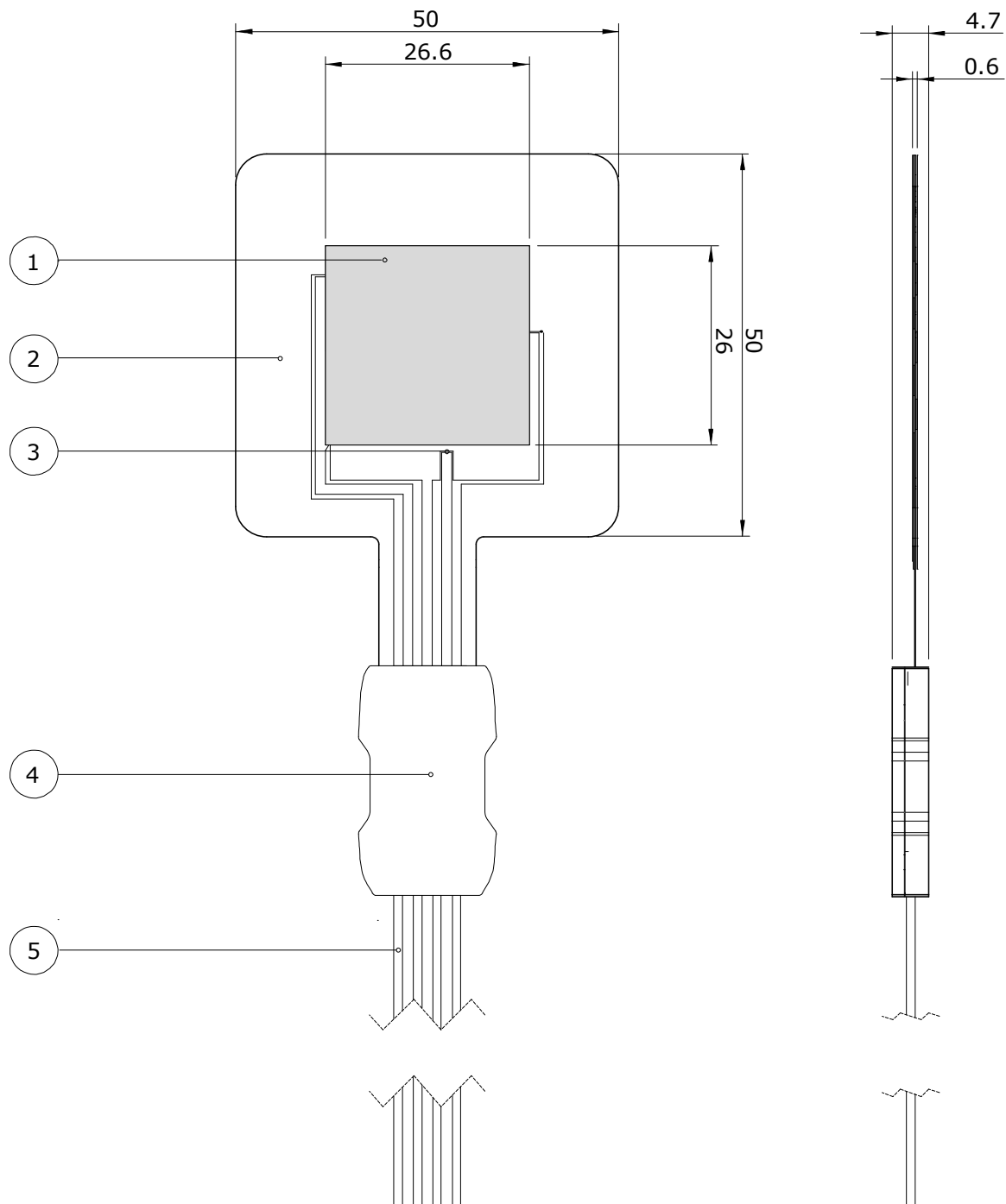
Figure 3.2.1 FHF01 heat flux sensor; dimensions in \times 10^{-3} m
