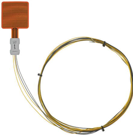
Figure 1.2.1 The HTR01 serial number is visible on the strain relief block. HTR01 is delivered with bundled wiring.
