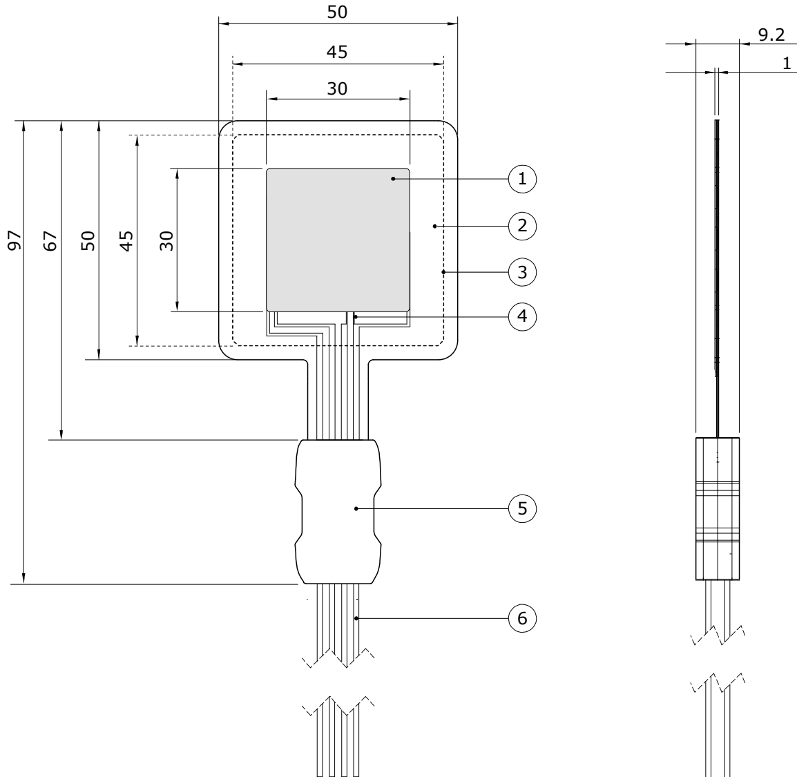
Figure 3.2.1 FHF02SC heat flux sensor; dimensions in \times 10^{-3} m
