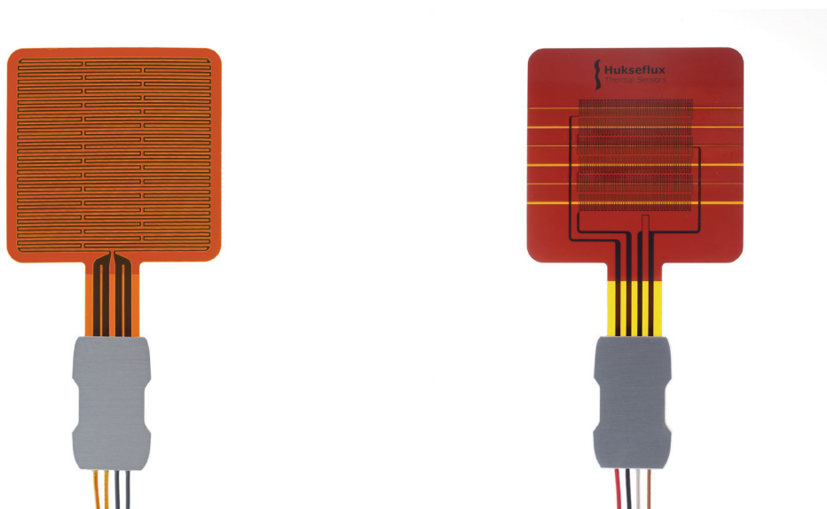
Figure 0.1 On the left HTR01 heater for calibration and verification of performance of FHF-type heat flux sensors, on the right an FHF01 heat flux sensor to which HTR01 may be applied. See also figure 3.2.1 for dimensions.
