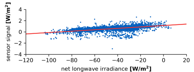
b) Nighttime offsets for an analogue Kipp & Zonen CMP22 pyranometer, externally ventilated and heated.
