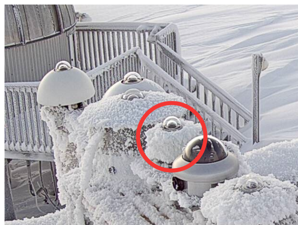
Figure 4 SR30 is battling the elements in Barrow, Alaska: the dome remains ice-free. Note that the neighbouring, completely ice-free sensors are heated with ten times more heating power. Picture taken on 27 JAN 2018 (temperature -30 °C), courtesy of NOAA.
